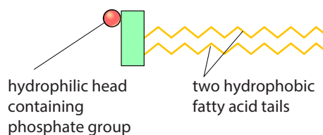
Figure 2.15: Diagrammatic representation of a phospholipid molecule. Compare this with Figure 2.13.
