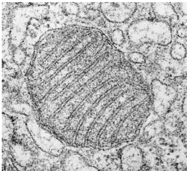
Figure 12.10: Transmission electron micrograph (TEM) of a mitochondrion ( \times 15000 ).
