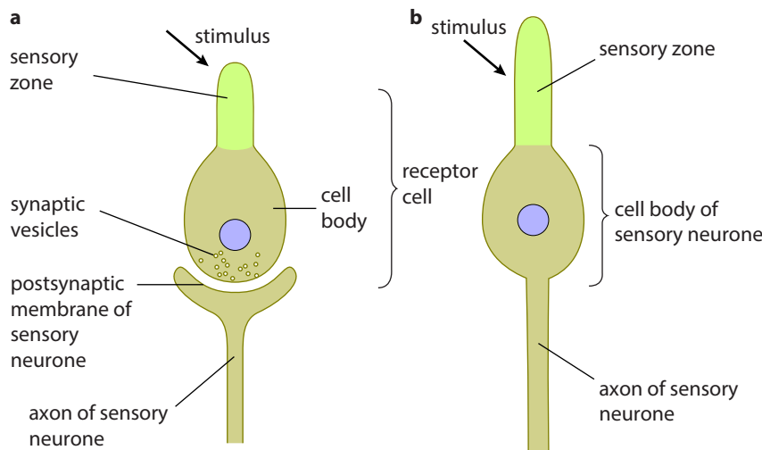
Figure 15.18: Receptors can be specialised cells a or simply the end of a sensory neurone b .
