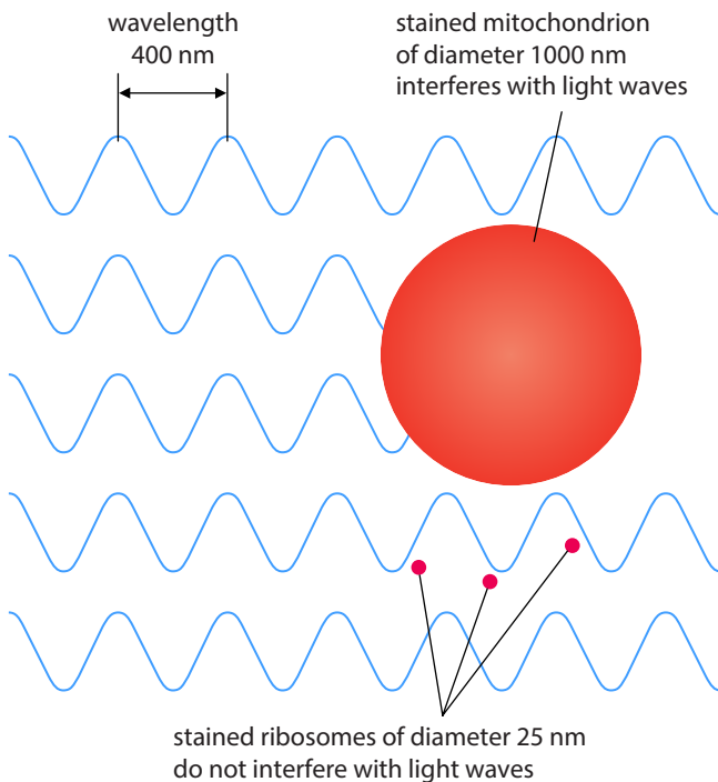
Figure 1.14: A mitochondrion and some ribosomes in the path of light waves of 400 \text{ nm} length.
