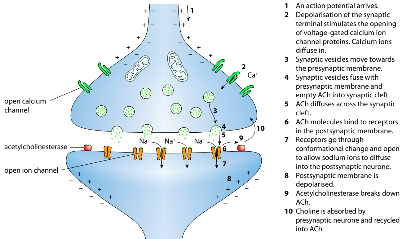
Figure 15.23: Synaptic transmission.
