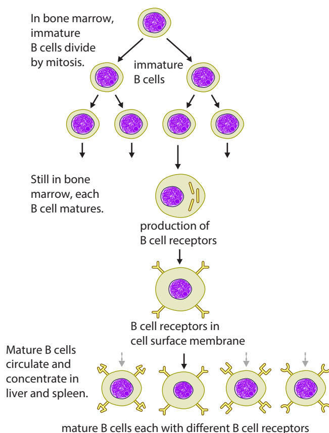
Figure 11.5: Origin and maturation of B-lymphocytes. As they mature in bone marrow, the cells become capable of secreting one type of antibody molecule with a specific shape. Some of these molecules become receptor proteins in the cell surface membrane and act like markers. By the time of a child's birth, there are millions of different B cells, each with specific B cell receptors. The diagram shows just four of these.
