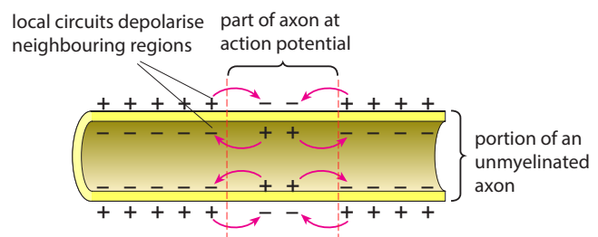
Figure 15.14: How an action potential passes along a neurone. The central part has been stimulated with an electrode to depolarise. The parts of the axon to left and right are at resting potential. Current flow (shown by arrows) depolarises the adjacent parts so impulses will pass along the axon in both directions away from the part stimulated.
