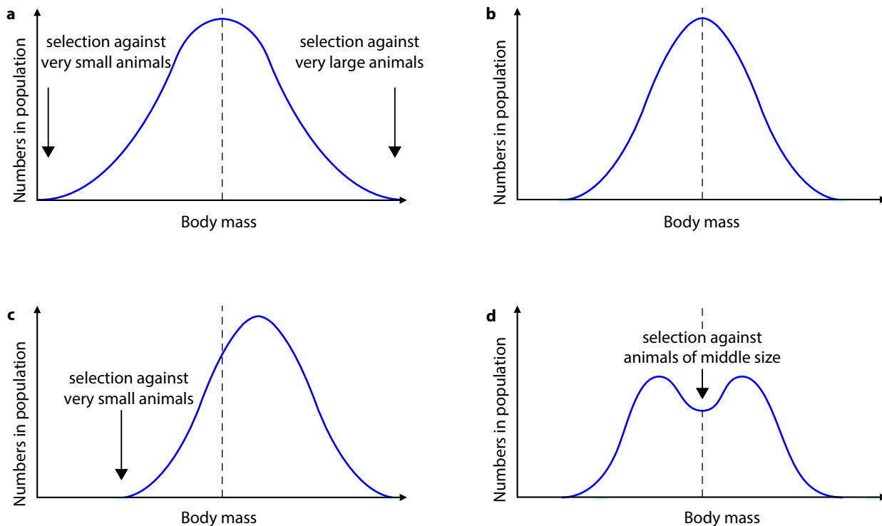
Figure 17.7: If a characteristic in a population, such as body mass, shows wide variation, selection pressures often act against the two extremes (graph a ). Very small or very large individuals are less likely to survive and reproduce than those whose size lies nearer the centre of the range. This results in a population with a narrower range of body size (graph b ). This type of selection, which tends to keep the variation in a characteristic centred around the same mean value, is called stabilising selection . Graph c shows what would happen if selection acted against smaller individuals but not larger ones. In this case, the range of variation shifts towards larger size. This type of selection, which results in a change in a characteristic in a particular direction, is called directional selection . Graph d shows the result of selection that favours both large and small individuals but acts against those whose size is in the middle of the range. This is disruptive selection .
