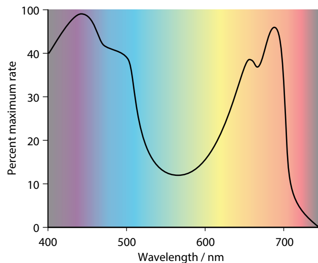
Figure 13.7: Action spectrum for photosynthesis.
