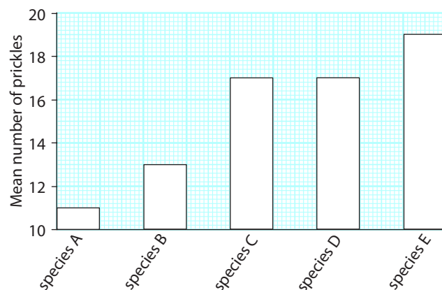
Figure P1.7: Bar chart showing the mean number of prickles on leaves from five different species of tree.
