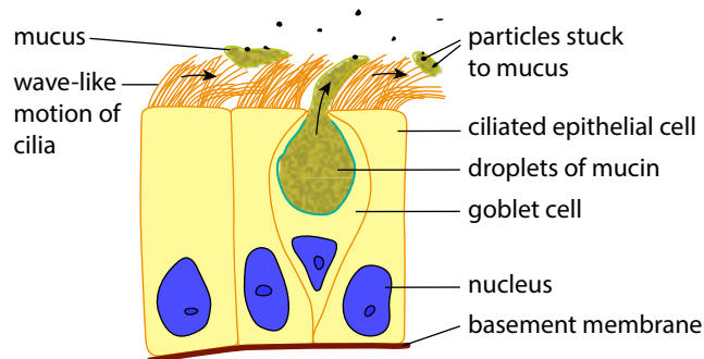
Figure 9.5: The wave-like beating of the cilia moves mucus secreted by goblet cells to the back of the throat.
