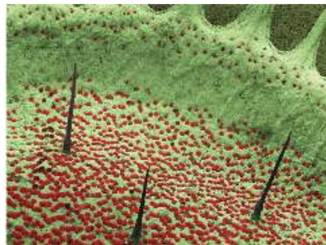
Figure 15.33: False-colour SEM of a leaf of a Venus fly trap with a group of stiff, sensitive hairs (black). When these are touched, the leaves respond by closing, capturing whatever was crawling over them. Enzymes are then secreted by glands (red) to digest the enclosed organism. Soluble products are absorbed by the leaf cells ( \times 25 ).
