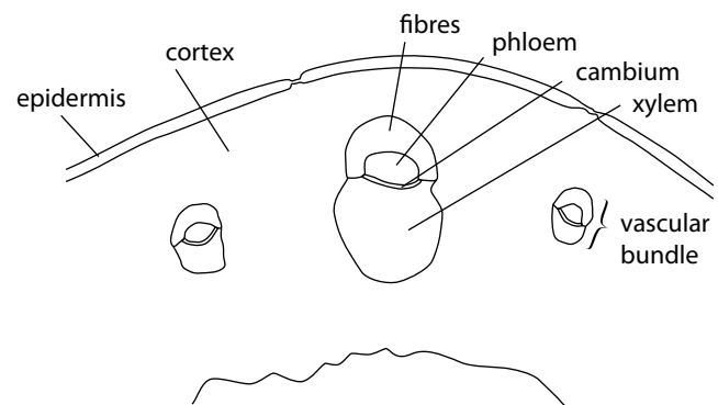
Figure 7.5: Low-power plan of the Ranunculus stem shown in Figure 7.4.
