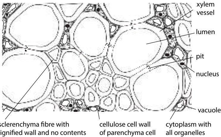
Figure 7.18: Structure of xylem. a Diagrams to show some different types of thickening in young xylem vessels. Young vessels (protoxylem) can still stretch longitudinally. b Photomicrograph of xylem as seen in LS ( \times 100 ). Lignin is stained red. LSs show the tube-like nature of the vessels. c and d Photomicrograph and diagram of xylem as seen in TS; lignin is stained red in c . Small parenchyma cells are visible between the xylem vessels in c and d ( \times 120 ). e Scanning electron micrograph of mature xylem vessels, showing reticulate (net-like) pattern of lignification ( \times 130 ).
