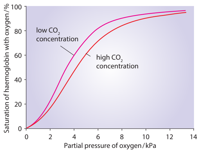
Figure 8.18: Dissociation curves for haemoglobin at two different partial pressures of carbon dioxide. The shift of the curve to the right when the haemoglobin is exposed to higher carbon dioxide concentration is called the Bohr shift.
