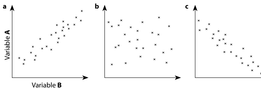
Figure 18.30: Three types of association: a a positive linear correlation; b no correlation; c a negative linear correlation.
