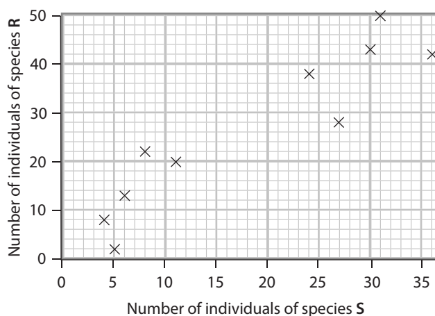
Figure P2.9: Scatter graph of the data in Table P2.5.
