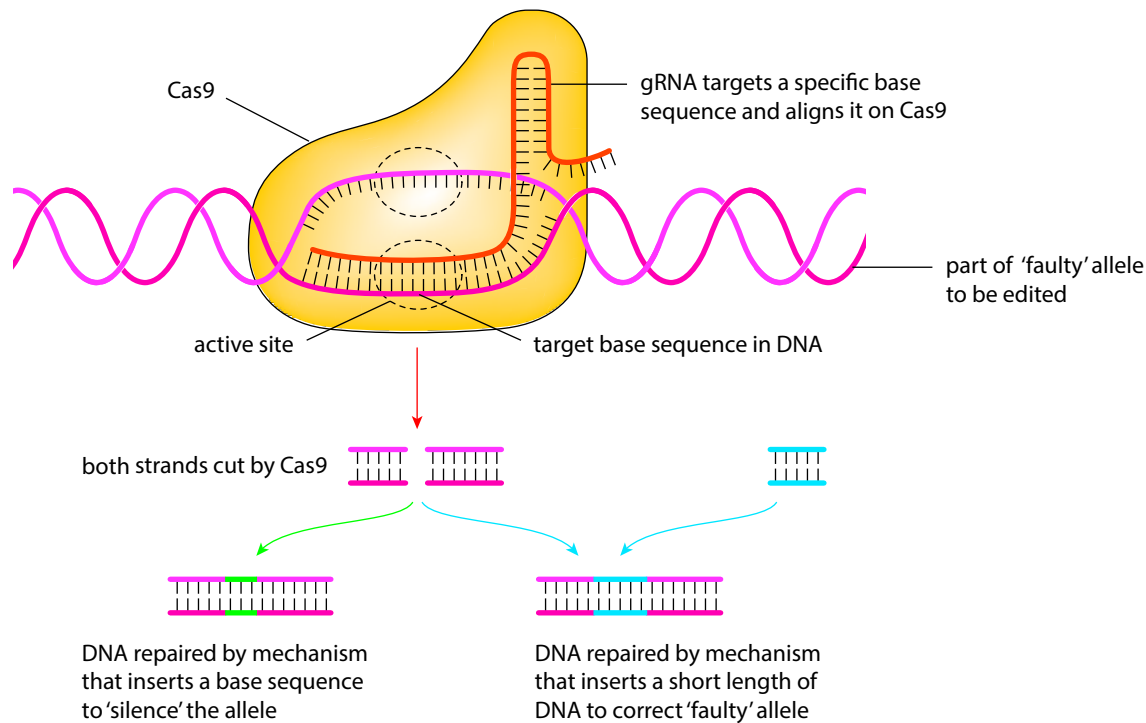
Figure 19.10: Gene editing using the Crispr/Cas9 system. Crispr is short for Clustered Regularly Interspaced Short Palindromic Repeats.
