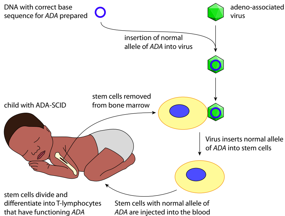
Figure 19.27: The procedure for carrying out gene therapy for SCID.
