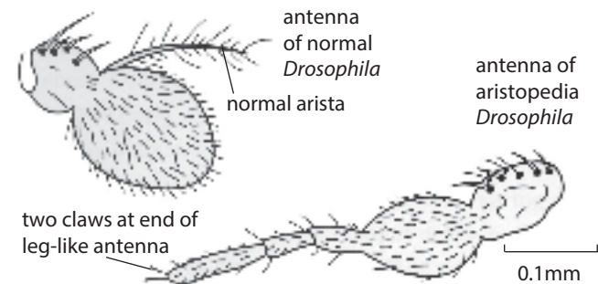
Figure 16.9: Normal and aristopedia Drosophila antennae.
