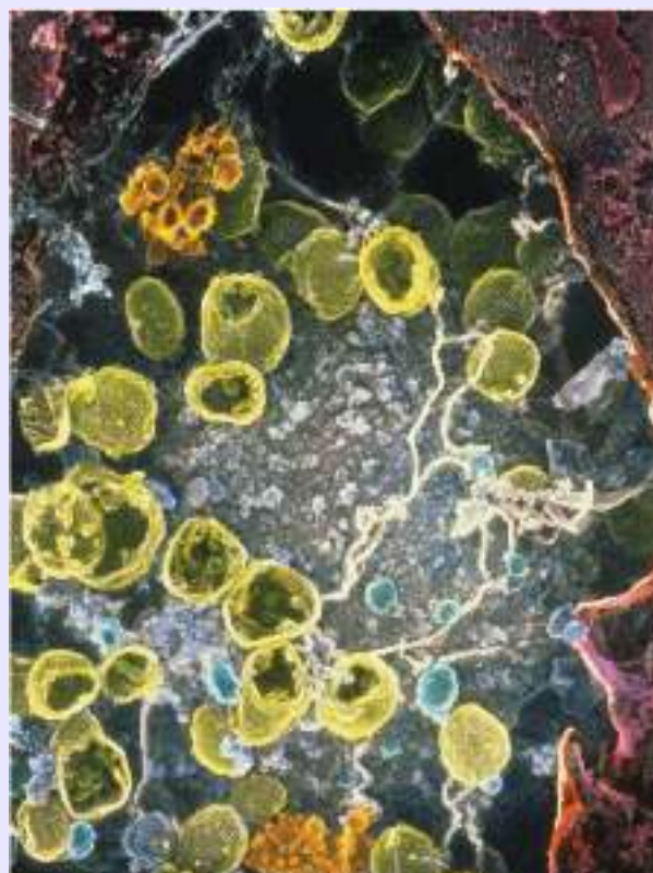
Figure 12.1: Scanning electron micrograph of a section through a human egg cell. The mitochondria have been coloured yellow ( \times 6000 ).
