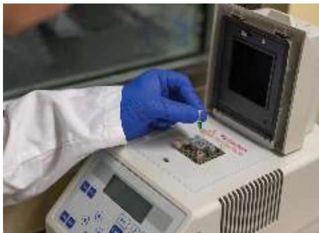
Figure 19.14: Loading a PCR machine (thermocycler) with the reagents needed to amplify small samples of DNA. The machine automatically changes the temperature of the mixtures in each tube. After 30 cycles in this machine there are 2 billion copies ( 2^{30} ) of the original DNA.
