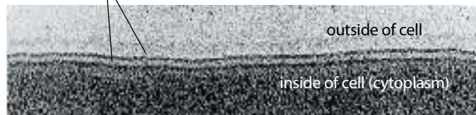
Figure 1.22: Cell surface membrane ( \times 250\,000 ). At this magnification the membrane appears as two dark lines at the edge of the cell.
