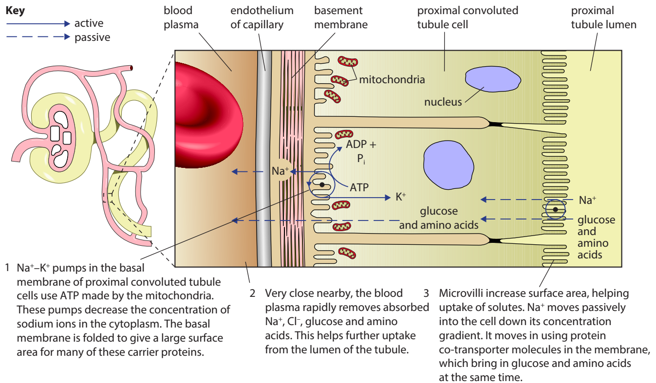
Figure 14.12: Reabsorption in the proximal convoluted tubule. As well as \text{Na}^+ - \text{K}^+ pump proteins, the basal membrane has many transport proteins for the facilitated diffusion of solutes, such as glucose and amino acids from the cells into the blood.
