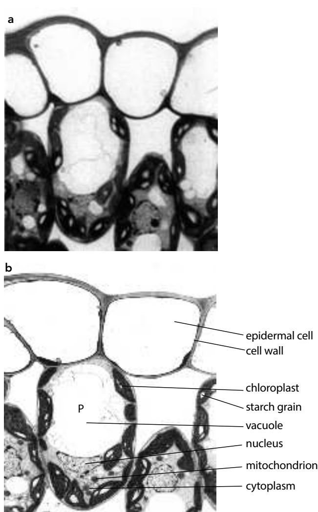
Figure 1.11: Micrographs of two sections of the same plant cells, as seen a with a light microscope, and b with an electron microscope. Both are shown at the same magnification (about \times 750 ).
