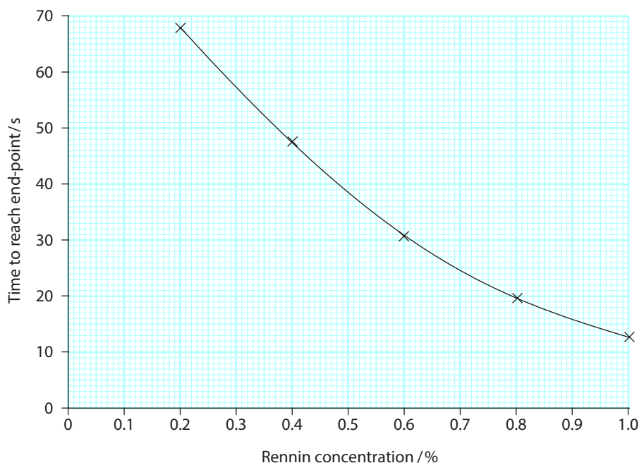
Figure P1.6: Line graph displaying the results in Table P1.1.
