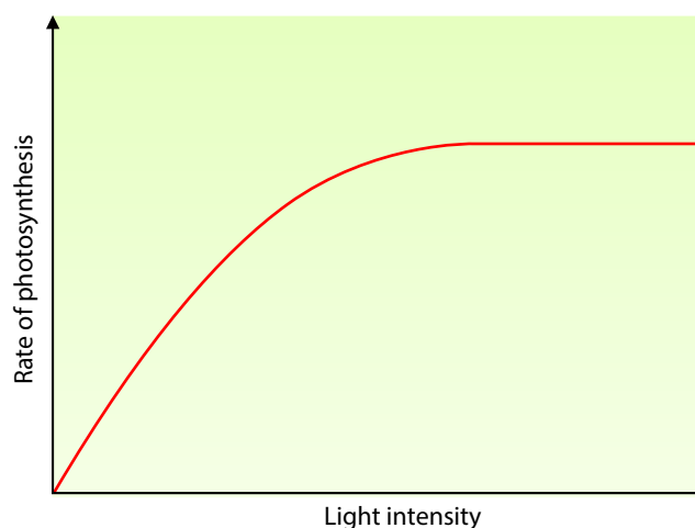
Figure 13.12: The rate of photosynthesis at different light intensities and constant temperature.
